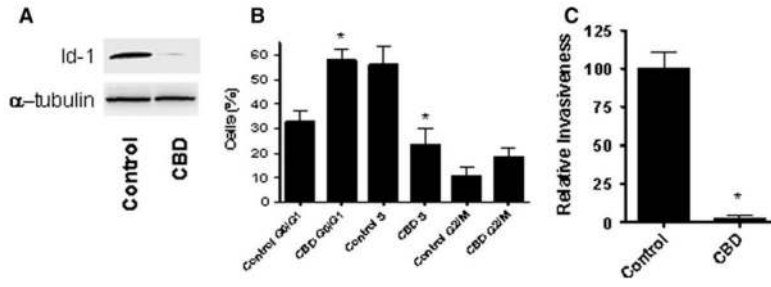
Fig. 4. CBD inhibits the expression of Id-1 and corresponding breast cancer proliferation and invasion in mouse 4T1 cells. (A) 4T1 cells were treated for 3 days with 1.5 \mu M CBD, proteins were extracted and analyzed for Id-1 expression. (B) 4T1 cells were collected and cell cycle analyzed using a desktop FACS Calibur with Cell Quest Pro software (BD Bioscience, CA). The distribution of cells in different cell cycle stages was determined according to their DNA content. (C) Invasion assays were carried out using the Boyden chamber assay. (*) indicates statistically significant differences from control ( P < 0.05 )
